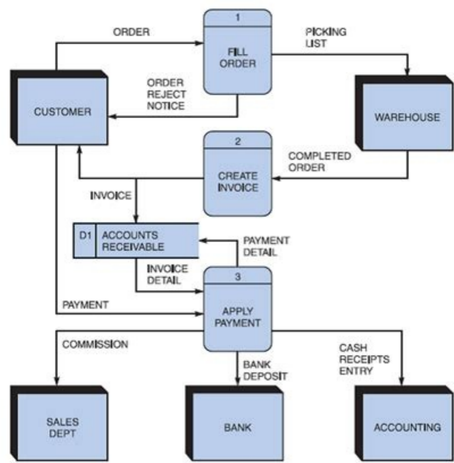
FIGURE 5-16 Diagram 0 DFD for the order system.
